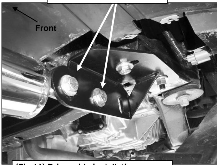
(Fig 11) Driver side installation pictured with lower bumper removed
