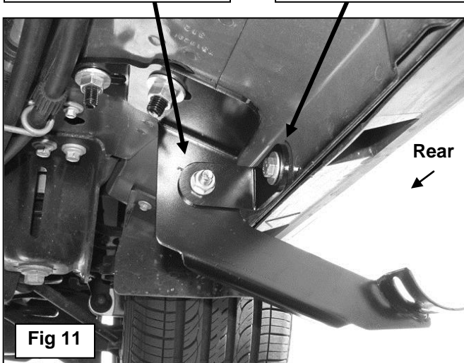
10mm x 30 Hex Bolt (2) 10mm Flat Washers 10mm Nylon Lock Nut
